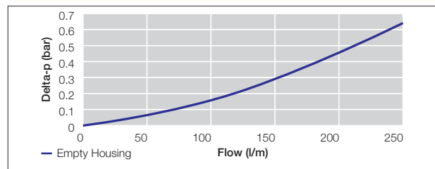
EPF Size 3 Empty Housing
