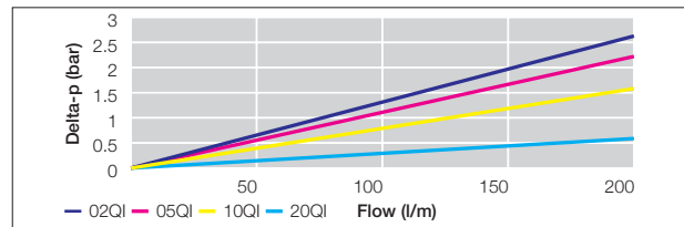
EPF Size 3 Length 1 Filter Elements
