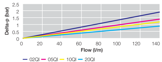
EPF Size 2 Length 2 Filter Elements with reverse flow valve
