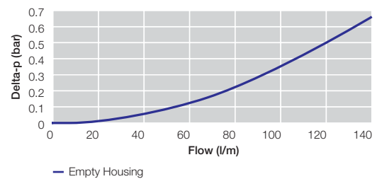
EPF Size 2 Length 2 Filter Elements
