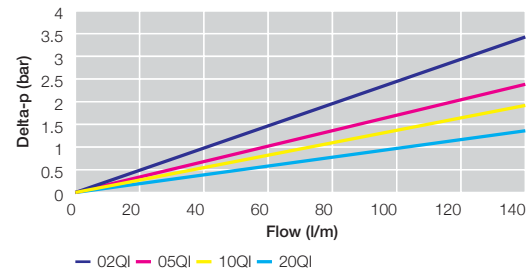
EPF Size 2 Length 1 Filter Elements with reverse flow valve
