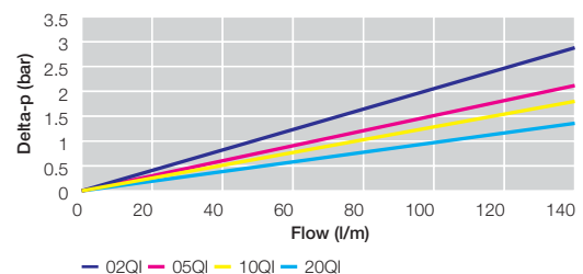
EPF Size 2 Length 2 Filter Elements with reverse flow valve
