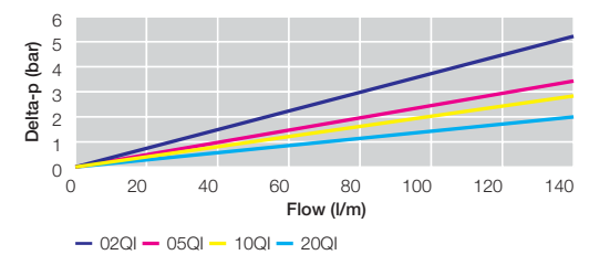
Empty Housing EPF Size 2
