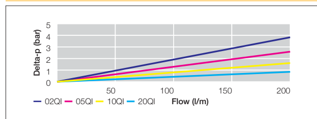
EPF Size 3 Length 1 Filter Elements with reverse flow valve
